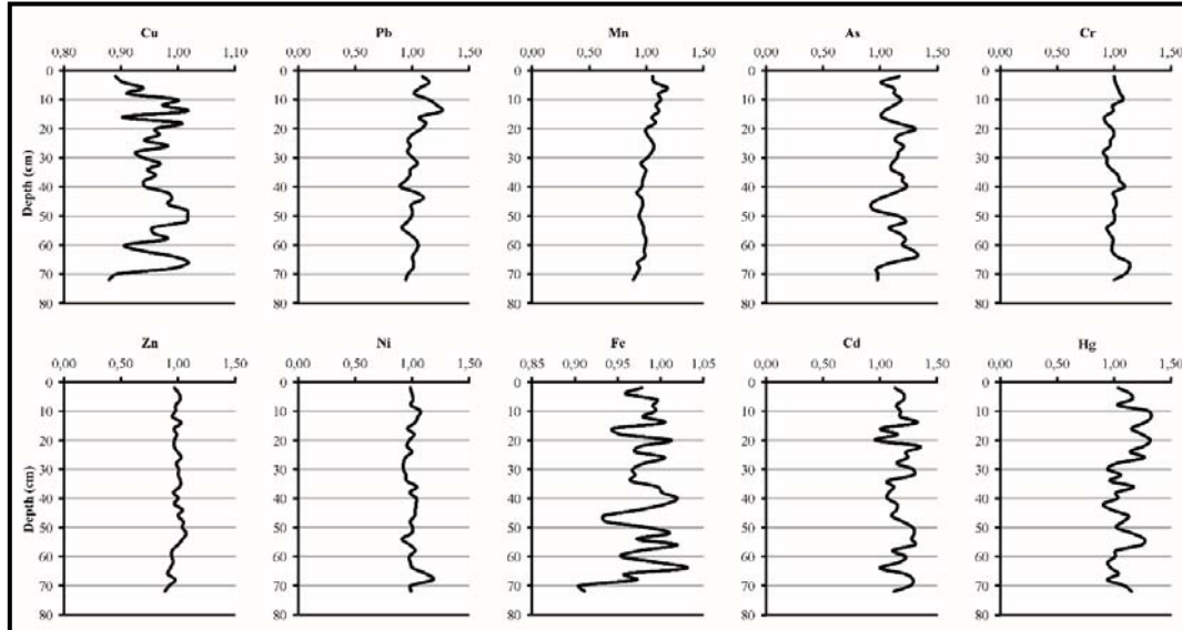
Fig.3. Vertical changes in enrichment factor values of heavy metals found in shallow sediment core sample from Lake Tortum.
