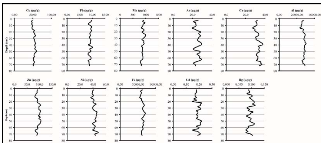
Fig. 2. Vertical distribution of heavy metals in core samples.
