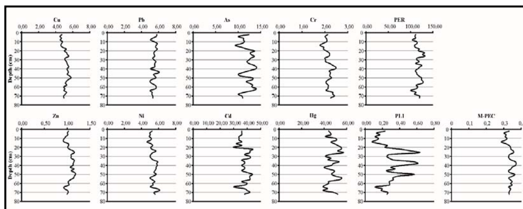
Fig.5. Vertical changes in integrated potential ecological risk (PER) and contamination load index of metals present in sediment of Lake Tortum.
