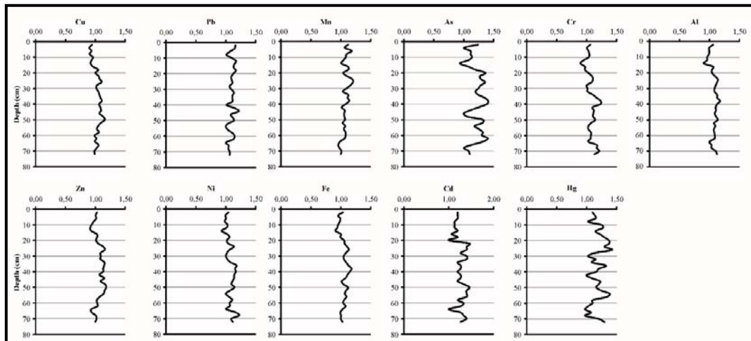
Fig.4. Vertical changes in contamination factor values of core sample from Lake Tortum.
